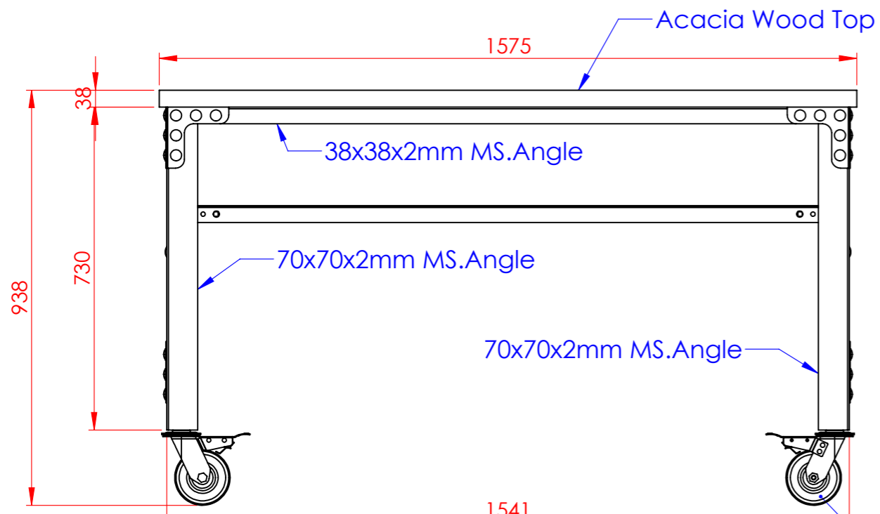
1541 Front View 1575
