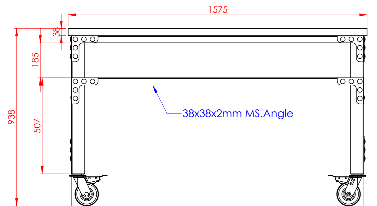
1541 Back View
